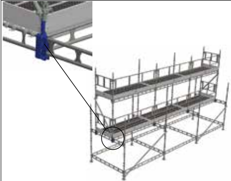
Puncheon Unit for Ledger Beams
